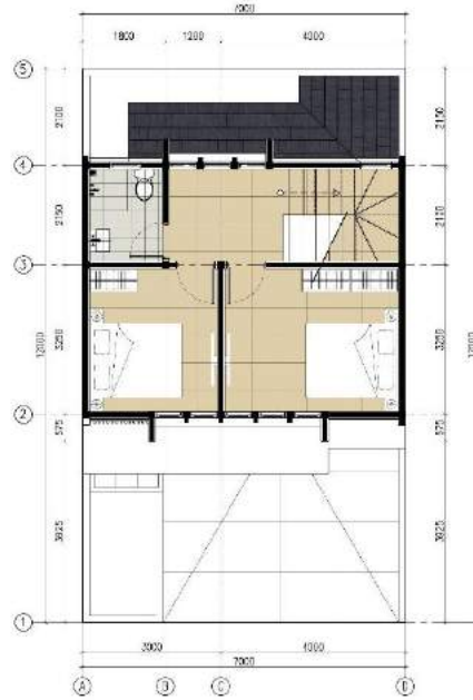
DENAH LT.02
