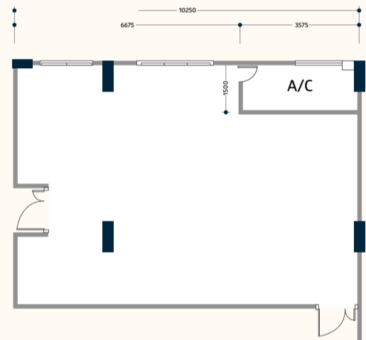
Type B Floor Area : 921 sq. ft. Location : Block A Ground Floor
