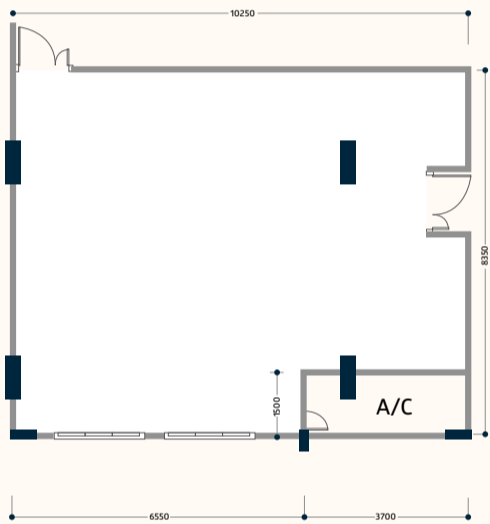
Type B Floor Area : 921 sq. ft. Location : Block A Ground Floor
