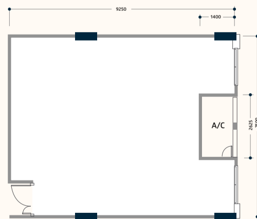
Type G Floor Area : 746 sq. ft. Location : Block B First Floor
