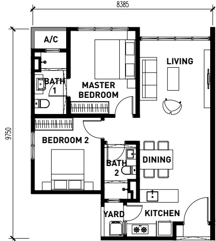
TYPE A2 788 sq.ft. 2 bedrooms | 2 bathrooms
