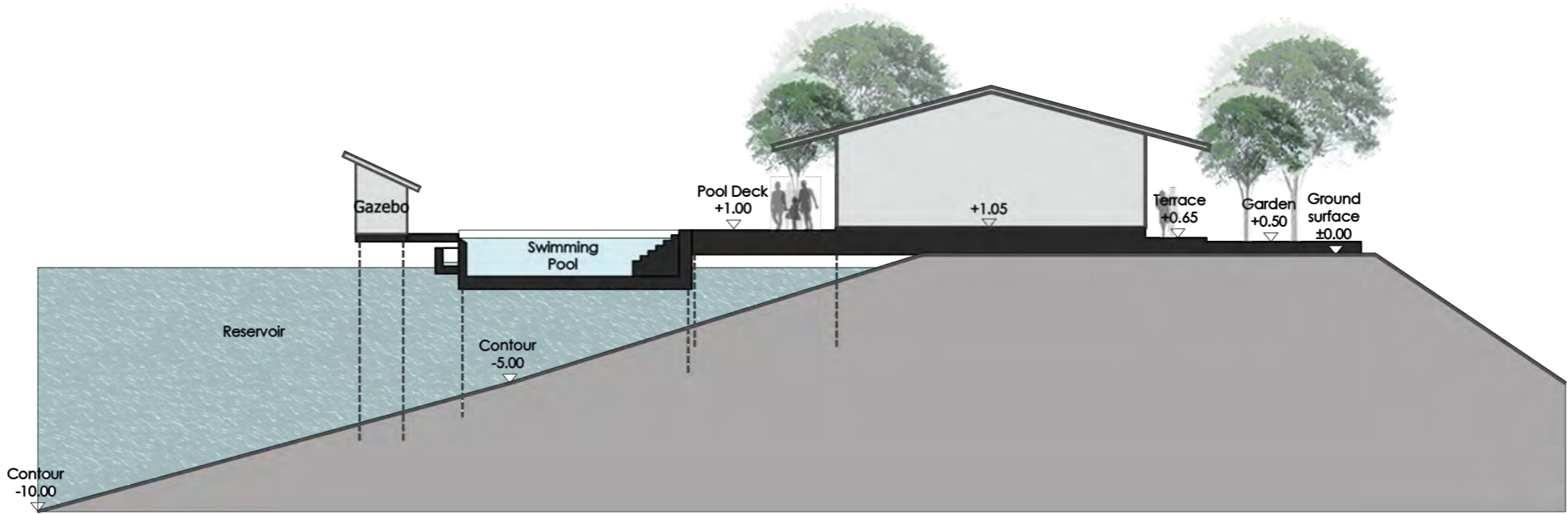
Principal Section
