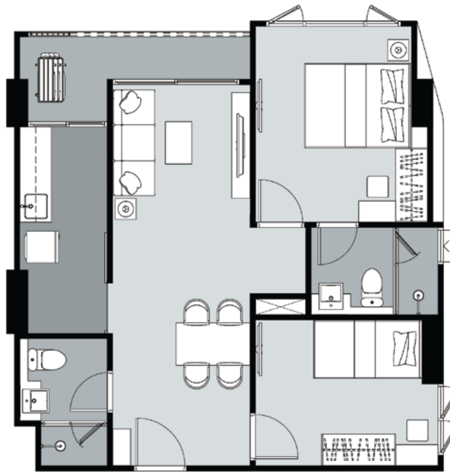
2D2 63.0 sq.m. 2 Bedrooms
