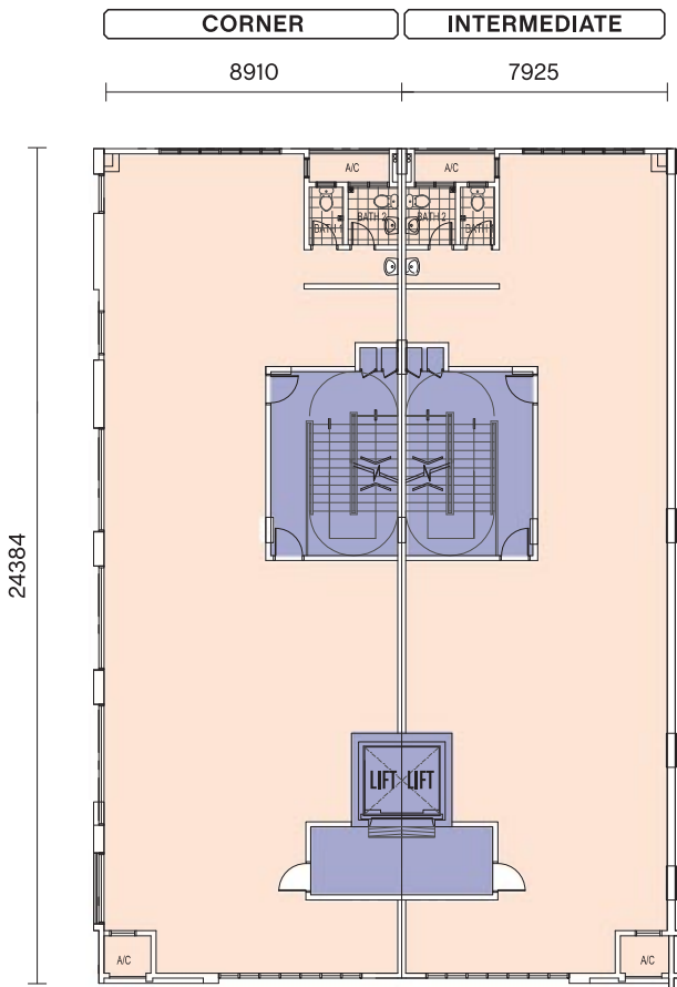
1st - 4th Floor 楼
