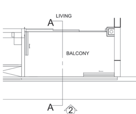
#44-01, #44-02, #44-04, #44-06, #44-08, #44-09, #44-10, #44-11, #44-12: TYPICAL RETRACTABLE BALCONY SCREEN (OPEN) - PLAN
