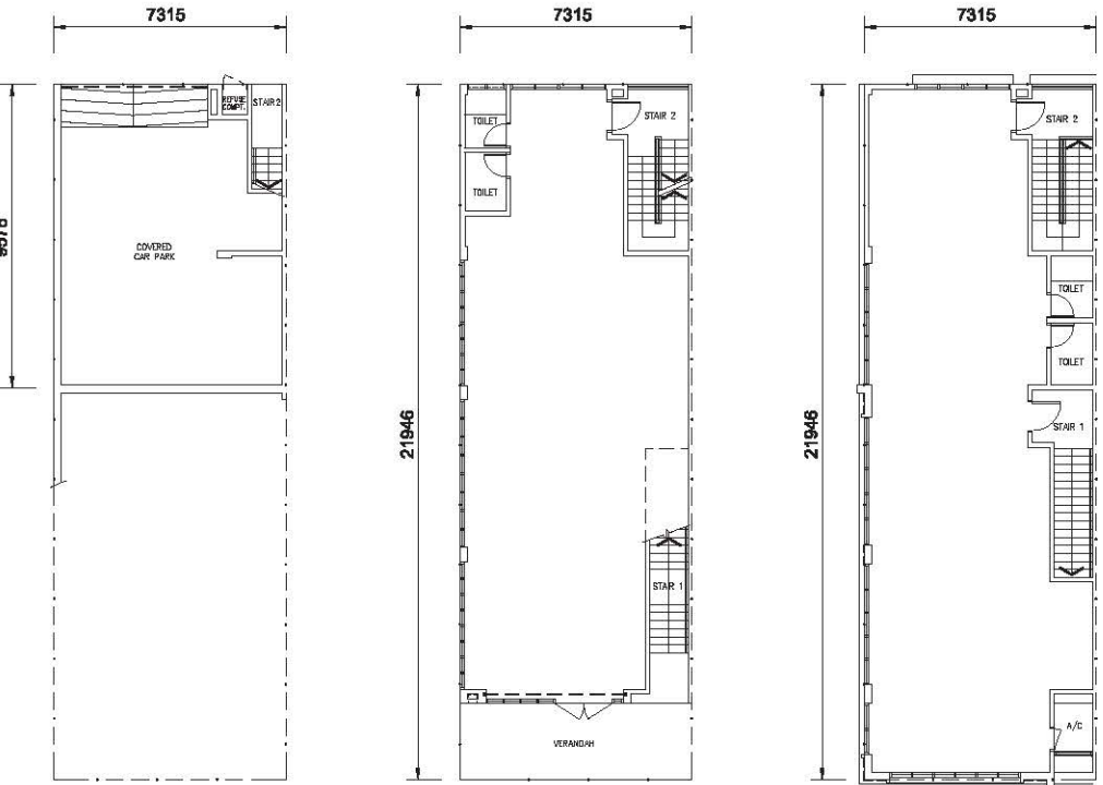
SUB-BASEMENT FLOOR PLAN
