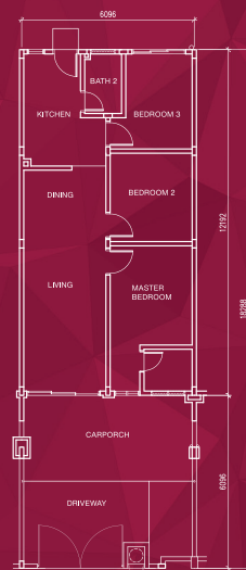
Ground Floor Plan Standard Intermediate Lot
