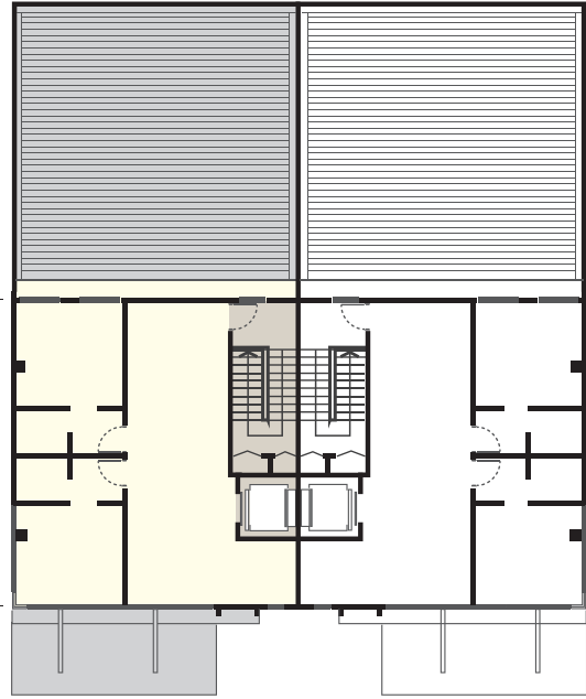
SECOND FLOOR
